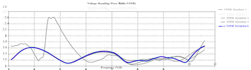
Figure 3.12 VSWR result in Simulation
