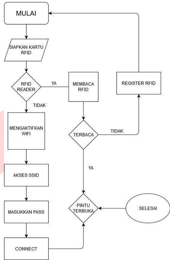
Gambar 3.4 Flowchart
