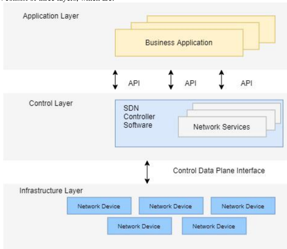
Fig. 1. SDN architecture.
