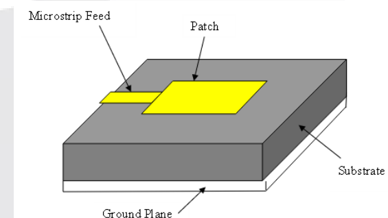
Gambar 2.5 Transmission feed line [12]
