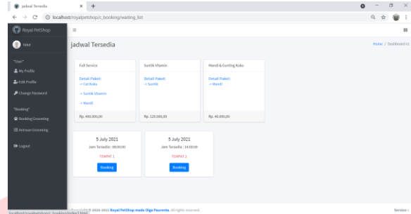
Gambar 4. 2 Halaman Booking
