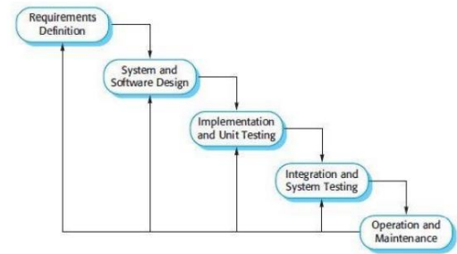
Gambar 1 . 1 SDLC Waterfall
