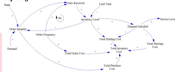
Figure IV. 1 Causal Loop Diagram Existing System
