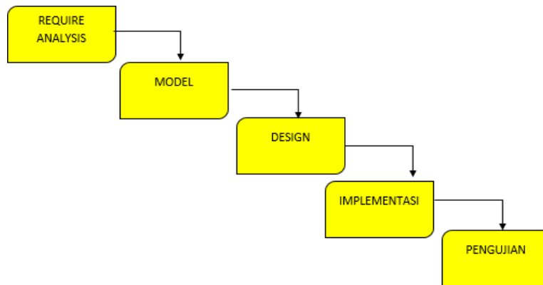
Gambar 3.1 Waterfall Diagram
