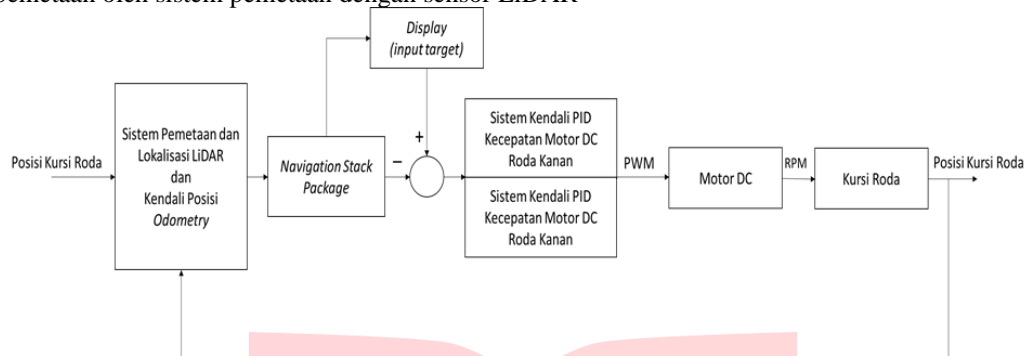
Gambar 3.1 Blok Diagram
