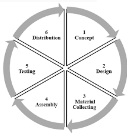
Gambar 3.1 Metode MDLC
