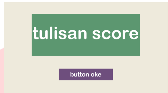
Gambar 3.8 Mockup Score
