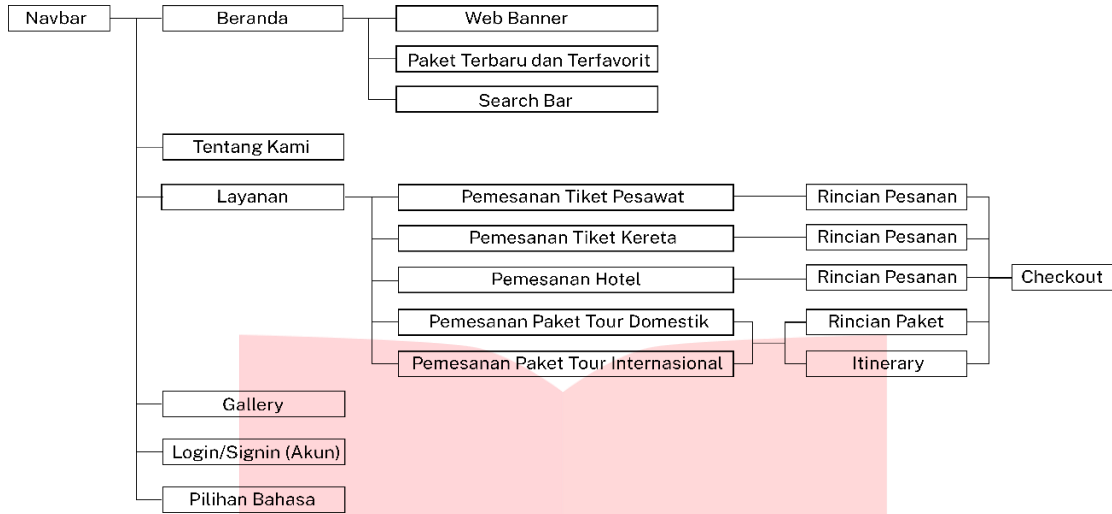
Gambar 1 (Flowchart Website)
