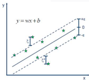
GAMBAR 2.3 MODEL SUPPORT VECTOR REGRESSION LINIER [8]
