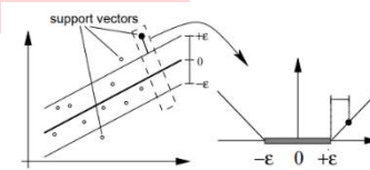
GAMBAR 2.2 FUNGSI SUPPORT VECTOR REGRESSION [11]
