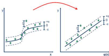
GAMBAR 2.4 MODEL SUPPORT VECTOR REGRESSION NON-LINIER [8]
