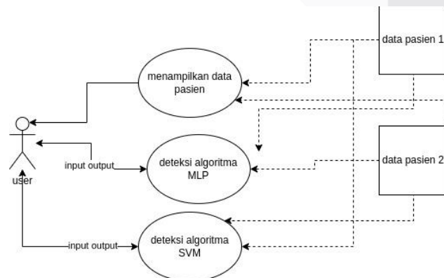
GAMBAR 2. 4 USE CASE
