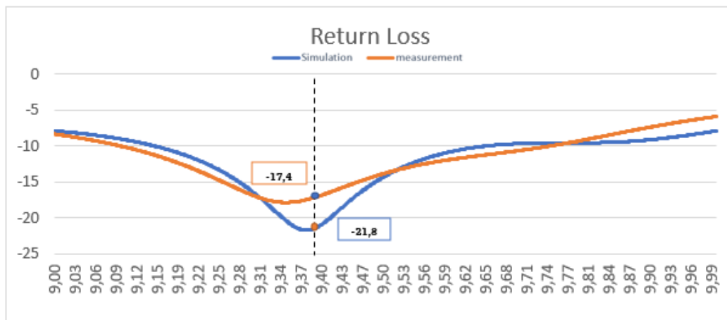
GAMBAR 7 NILAI RETURN LOSS
