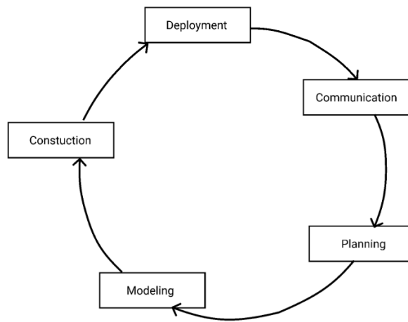
Gambar 1- 1 SDLC Prototype
