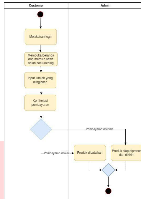
GAMBAR 4 ACTIVITY DIAGRAM
