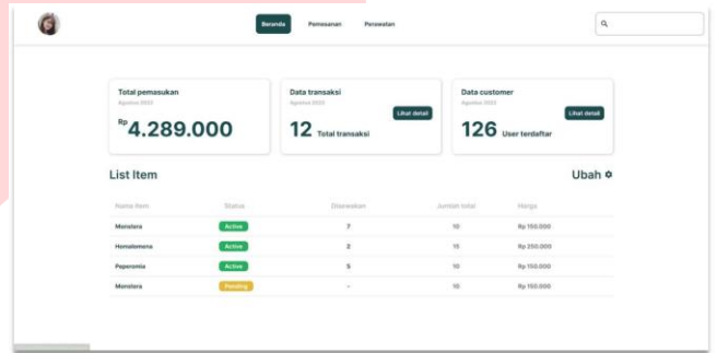
GAMBAR 10 BERANDA ADMINISTRATOR
