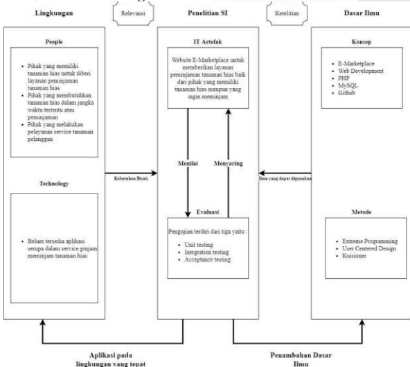
GAMBAR 1 MODEL KONSEPTUAL
