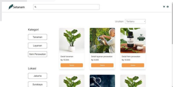
GAMBAR 12 BERANDA CUSTOMER
