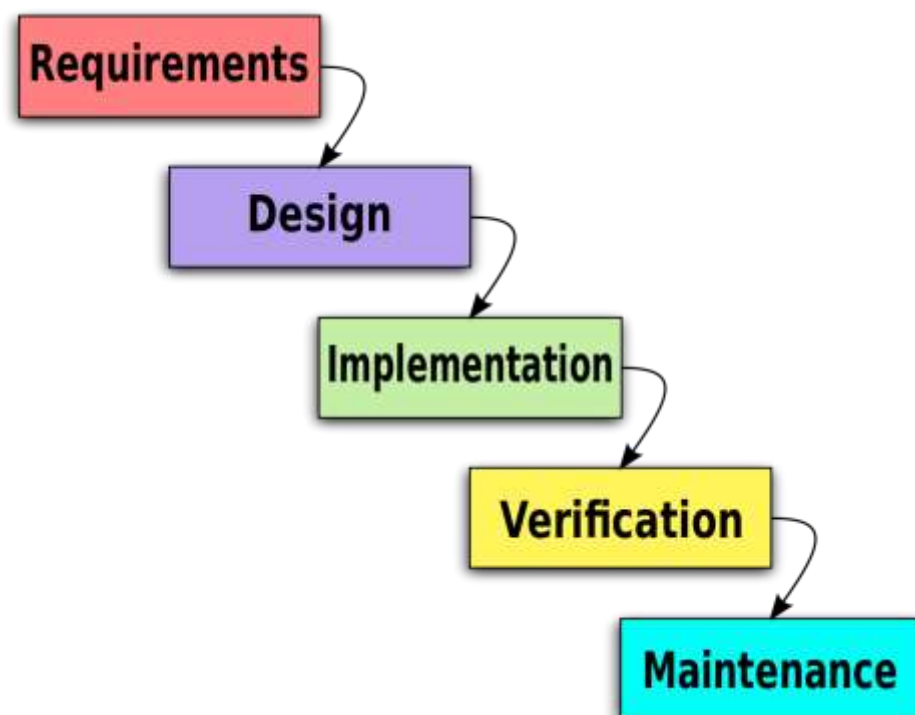
Gambar 1 Model Waterfall
