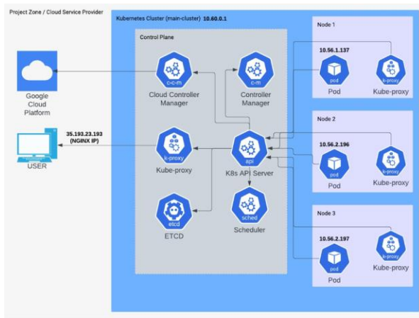
FIG. 1 THE PROPOSED SYSTEM DESIGN OF THE KUBERNETES CLUSTER DESIGN.
