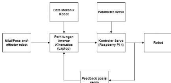
GAMBAR 7 Diagram Blok
