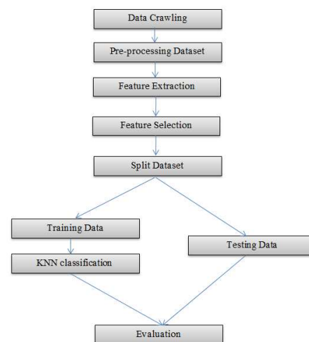
Figure 1. System Flowchart
