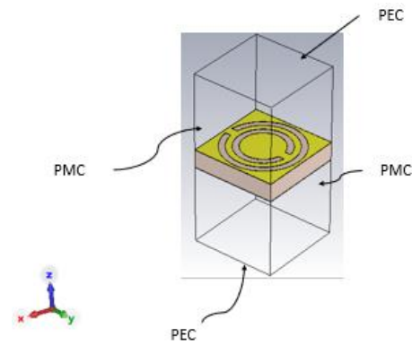
GAMBAR 9 unit cell CSRR
