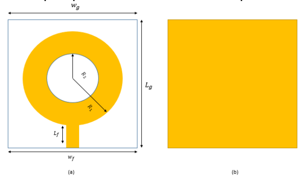
GAMBAR 5 Desain awal antenna mikrostrip patch circular ring
