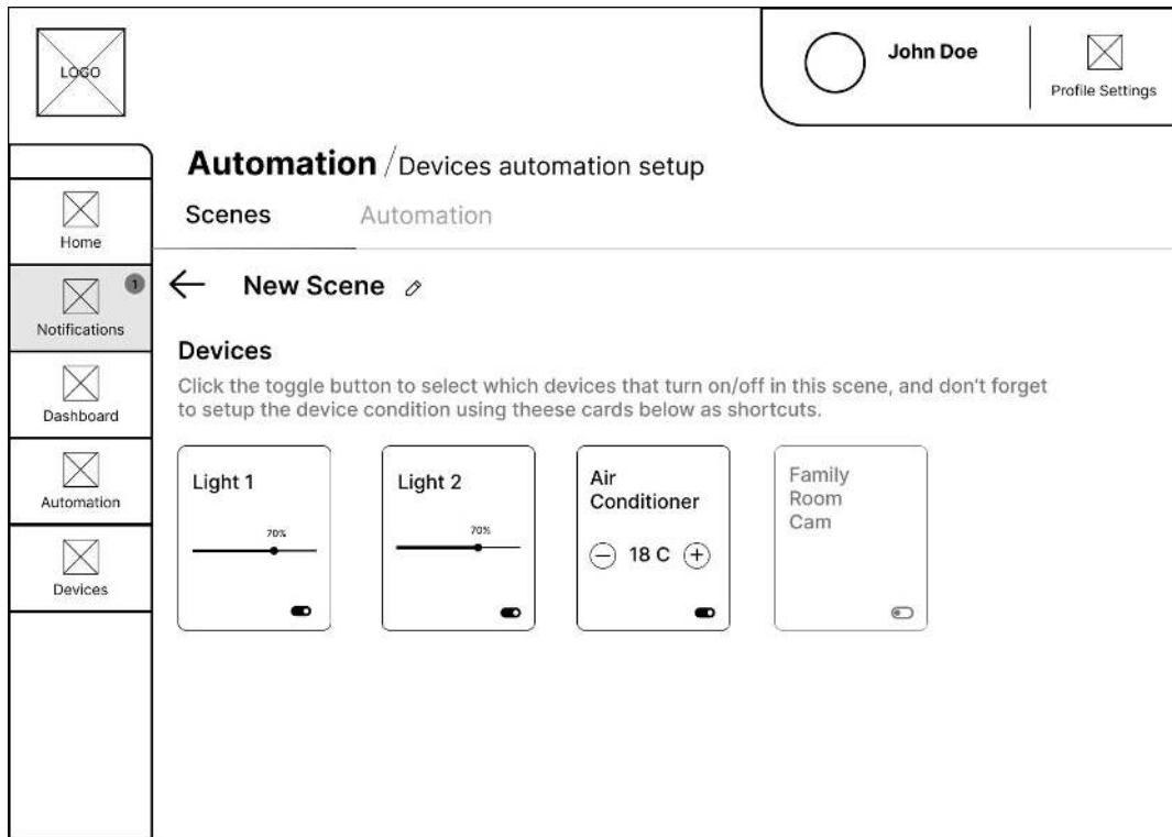
Gambar 26 Wireframe Automation 2
