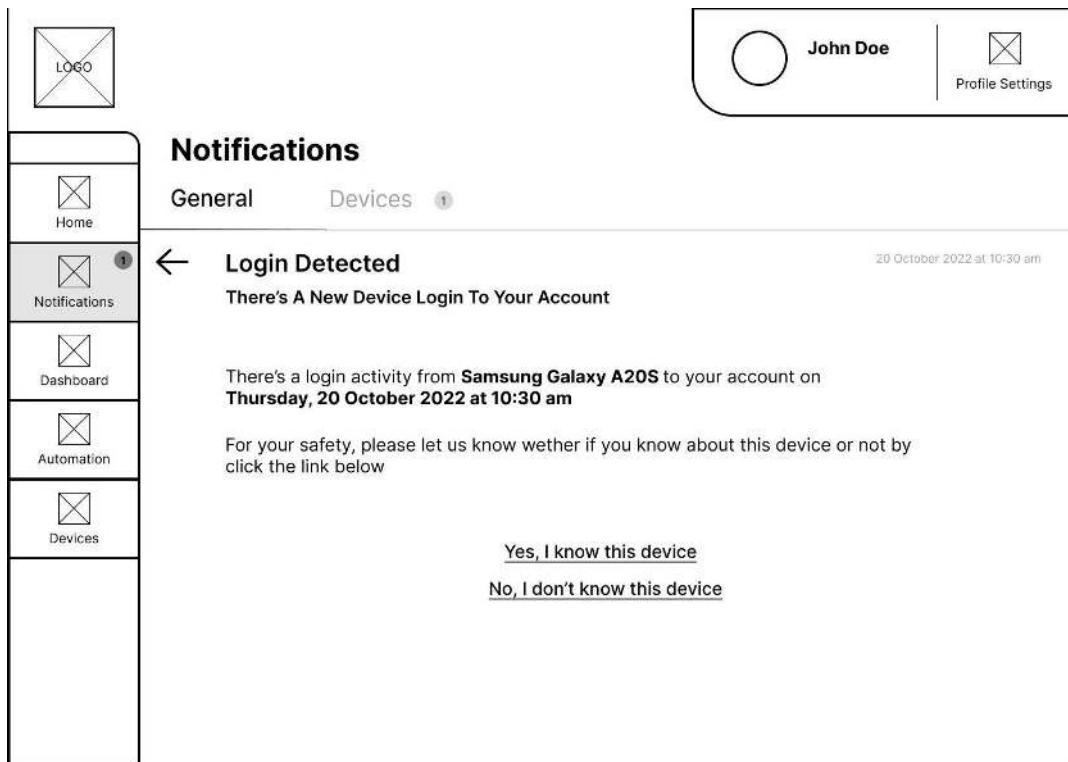
Gambar 23 Wireframe Notifications 2
