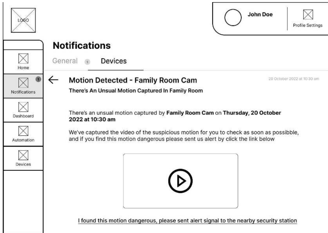
Gambar 24 Wireframe Notifications 3
