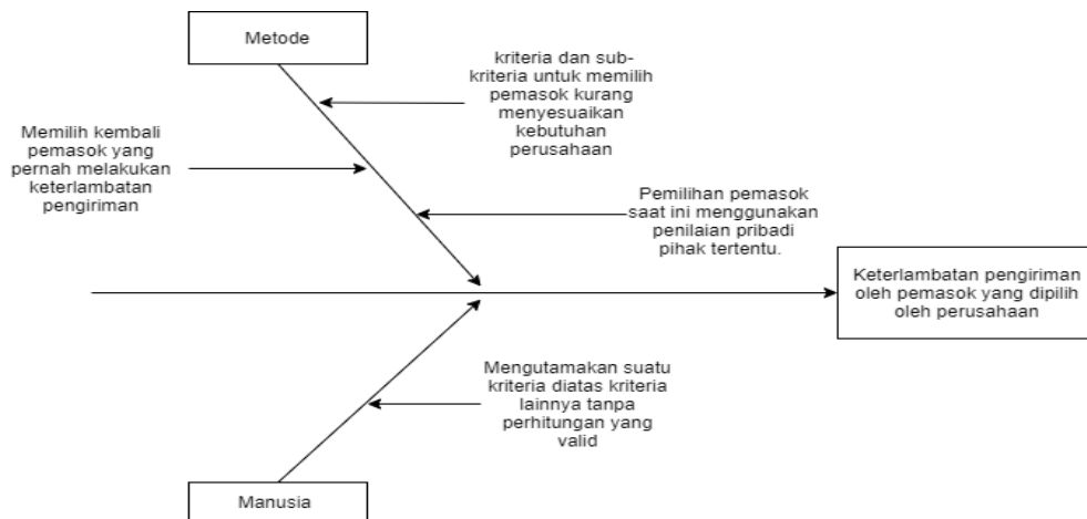
Gambar I. 2 Diagram Fishbone
