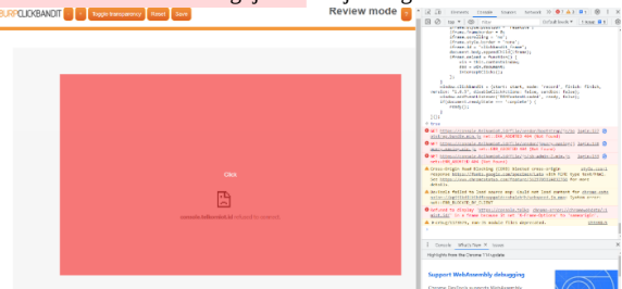
GAMBAR 4.8 Pengujian Clickjacking
