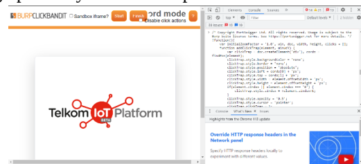
GAMBAR 4.7 Pengujian Clickjacking
