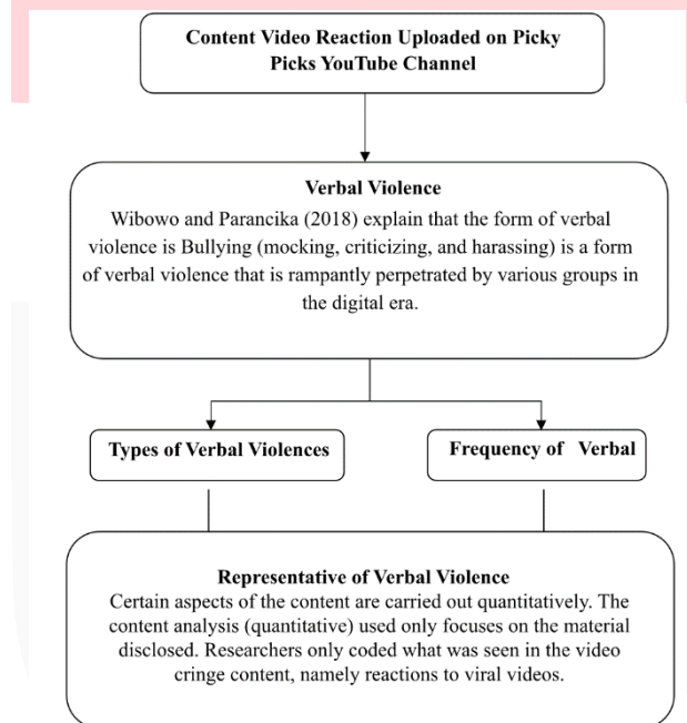
Figure 1. Framework
