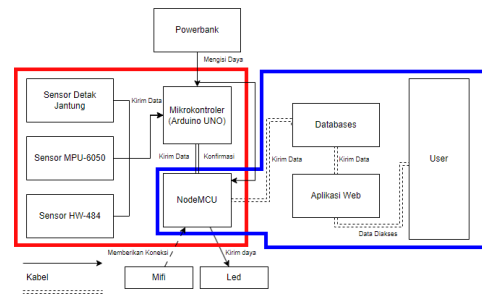
GAMBAR 1 Blok Diagram
