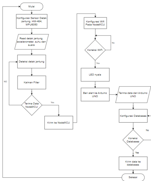
GAMBAR 2 Flowchart Program Hardware
