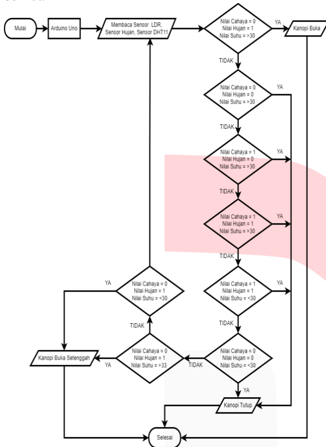
GAMBAR 7 (Flowchart)
