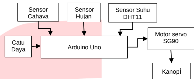
GAMBAR 6 (Diagram Blok)
