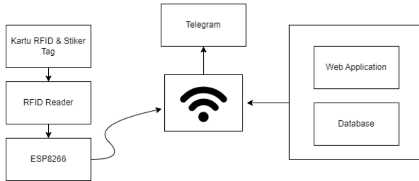
Gambar 2. Blok Diagram
