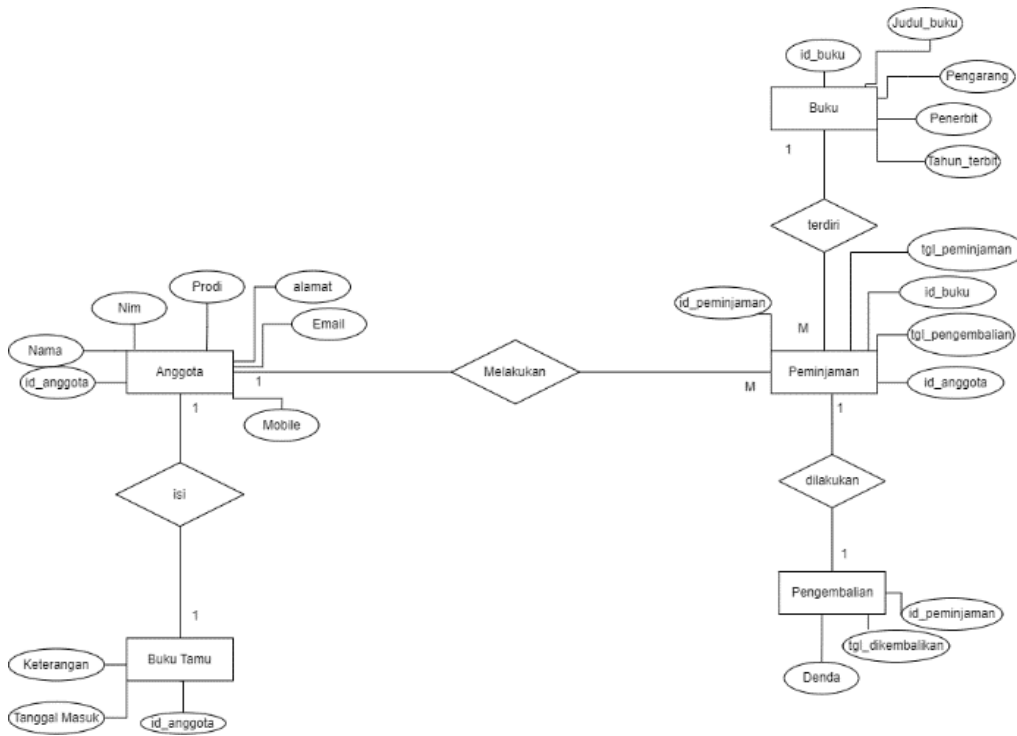
Gambar 5. ERD Diagram
