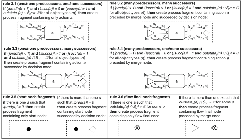
Fig. 5. Generating process fragments in step 3
