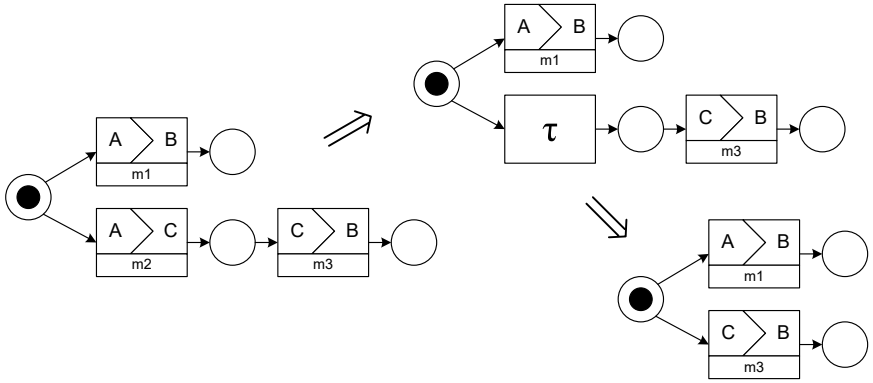
Fig. 4. \tau -transitions need to be removed
