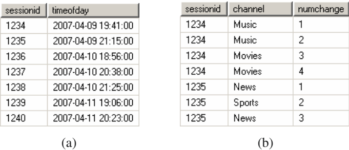
Fig. 1. Case (a) and nested (b) tables for the simple TV usage scenario
