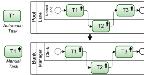
Fig. 3. Manual Tasks and Roles in BPMN
