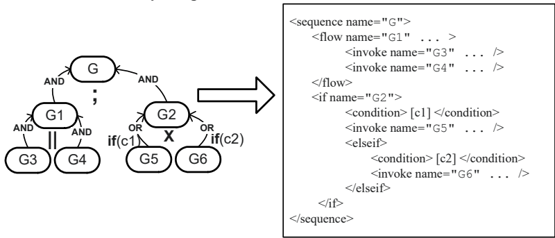
Fig. 5. Example of WS-BPEL 2.0 code generation
