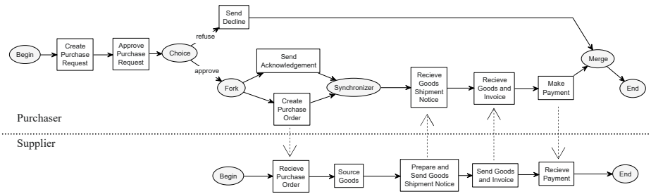
Fig. 3. Purchase-to-Pay Scenario
