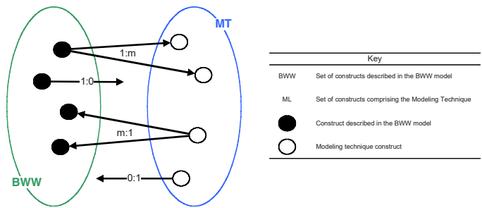
Fig. 1. Types of Potential Representational Deficiencies [4]
