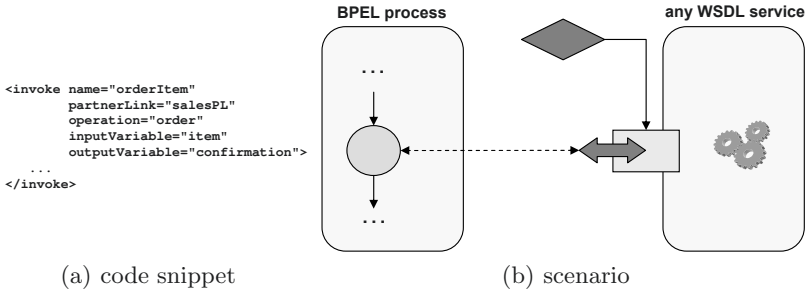
Fig. 4. Synchronous invocation of a WSDL service
