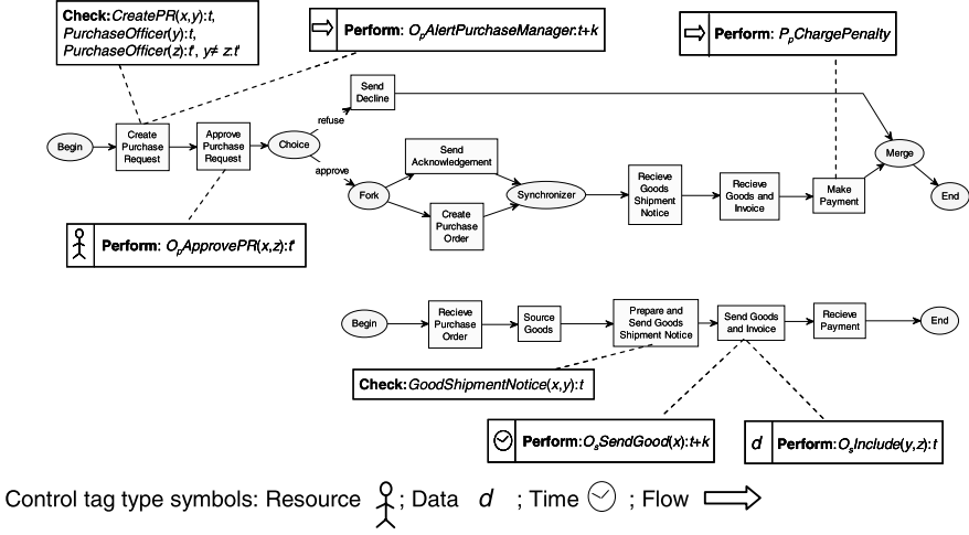
Fig. 4. Visualization of Control Tags
