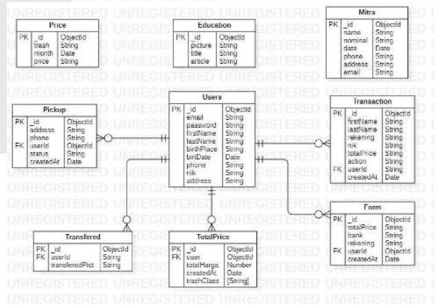
GAMBAR 1. Entity Relationship Diagram
