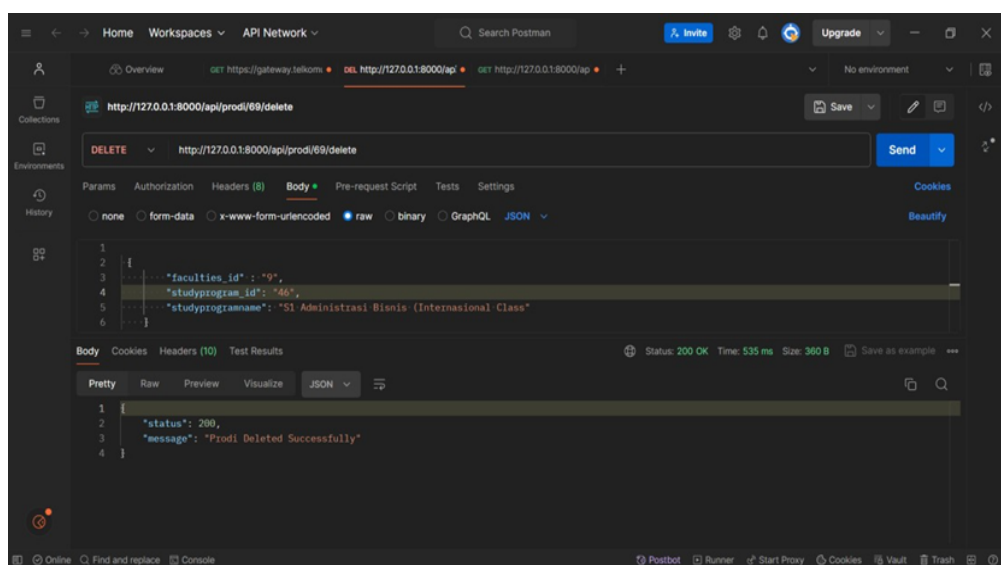
Gambar 2. 18 DELETE Prodi
