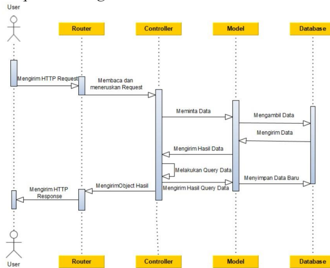
Gambar 2. 7 Sequence Diagram
