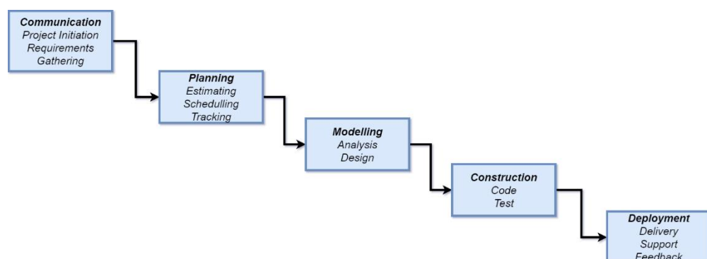
Gambar 1-1 Metode Waterfall
