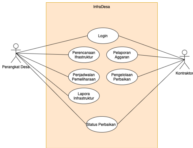
GAMBAR 32 Use Case Diagram InfraDesa
