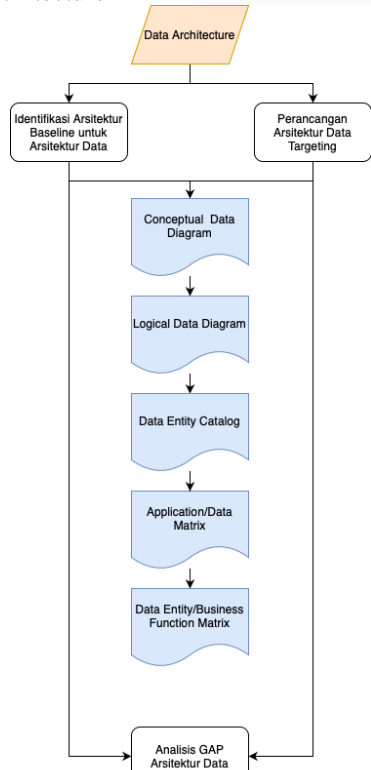
GAMBAR 8 Data Architecture
