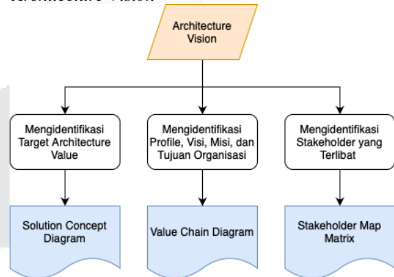
GAMBAR 6 Architecture Vision
