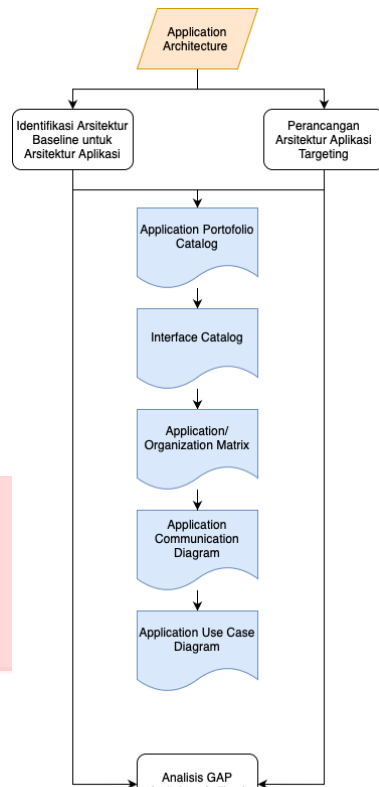
GAMBAR 9 Application Architecture
