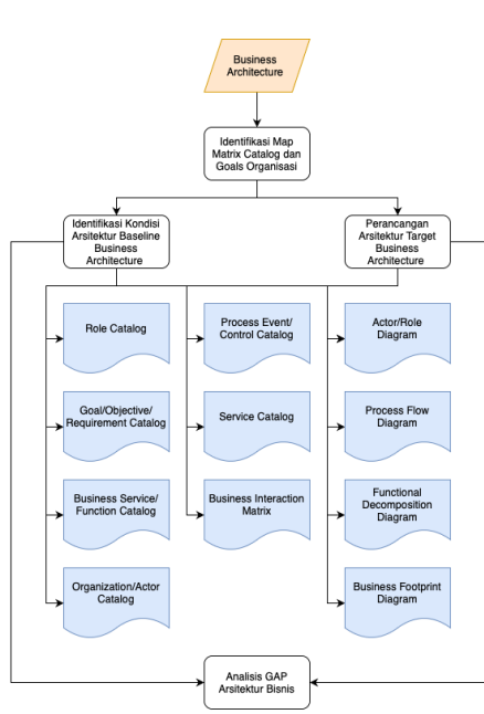
GAMBAR 7 Business Architecture
