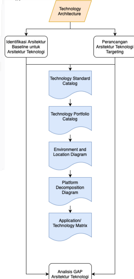
GAMBAR 10 Technology Architecture
