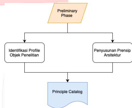
GAMBAR 5 Preliminary Phase
