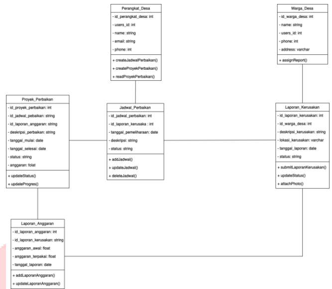
GAMBAR 27 Class Diagram InfraDesa
