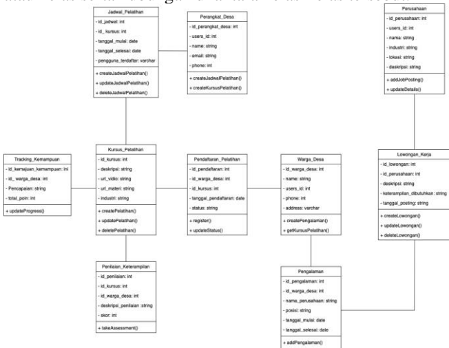
GAMBAR 26 Class Diagram JobMatch
