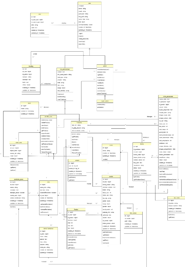
Gambar II-17 Class Diagram
