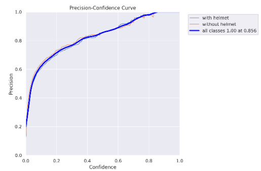
Gambar 14 Precision-Confidence curve
