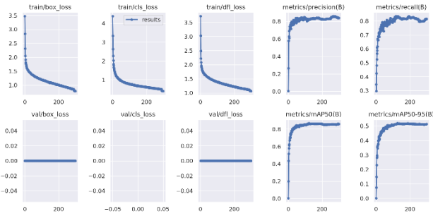
Gambar 16 Train Loss Result Curve
