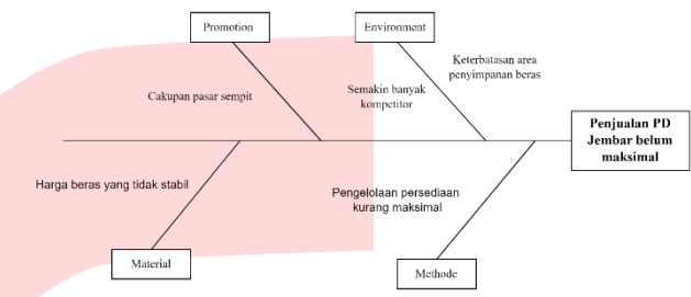
Gambar 3 Fishbone Diagram
