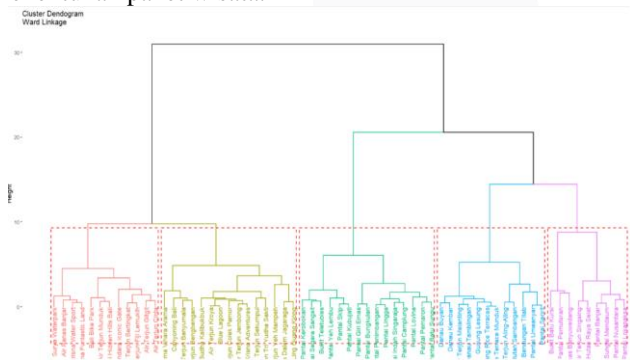
GAMBAR 4 Hasil Dendrogram
