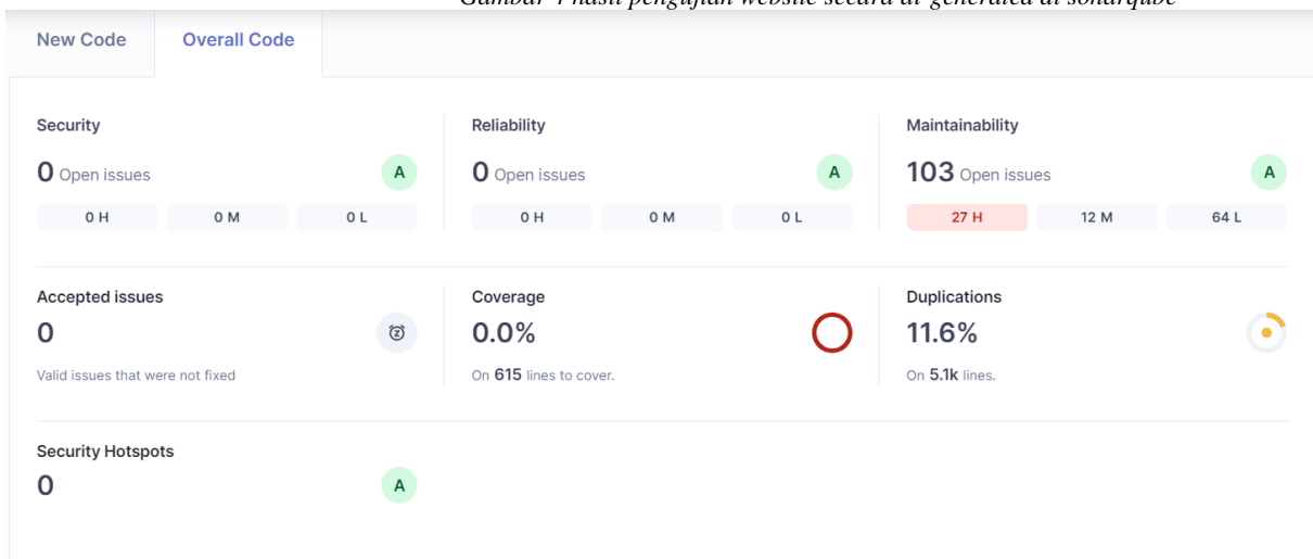
Gambar 4 hasil pengujian website secara ai-generated di sonarqube
