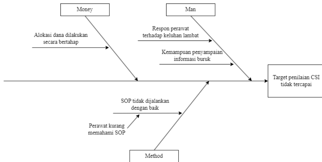
Gambar I. 2 Fishbone Diagram
