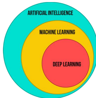
Gambar 3. Deep learning
