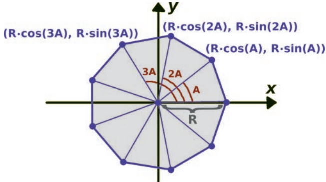
FIGURE 4.11 Calculating the vertices of a regular polygon.
