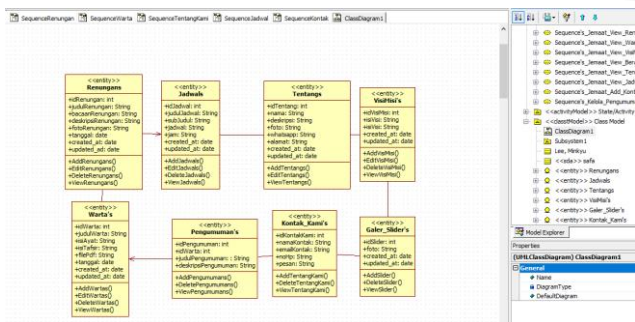
Gambar 1.3 Class Diagram
