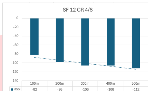
GAMBAR 19 (Grafik RSSI SF 12 CR 4/8)
