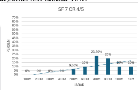
GAMBAR 20 (Grafik Packet Loss SF 7 CR 4/5)
