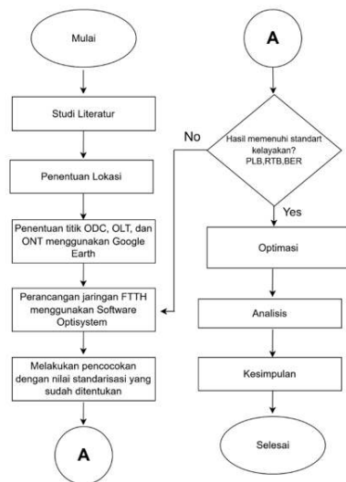
GAMBAR 9 (ALUR PENELITIAN)
