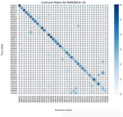
GAMBAR 4 Confussion Matrix Hasil Skenario 1
