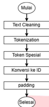
GAMBAR 7 Alur Tokenizing
