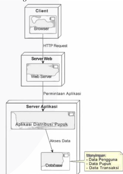
Gambar 10. Deployment Diagram
