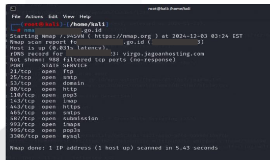
GAMBAR 4 Hasil Scanning Nmap
