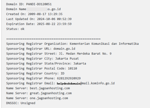
GAMBAR 3 Hasil Whois Lookup
