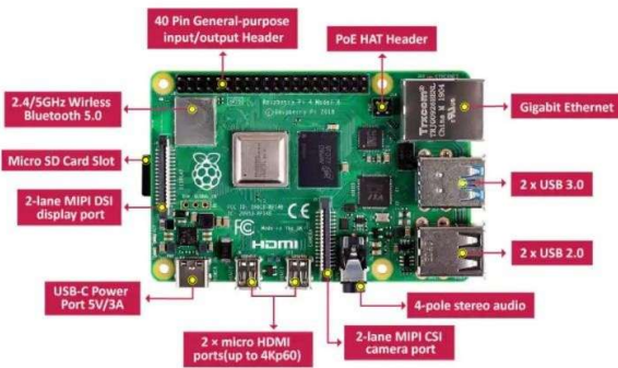
GAMBAR 2.1 Raspberry pi
