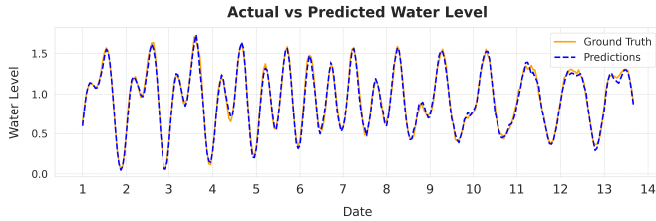
Fig. 6: iTransformer 14-days Actual and Prediction Data.
