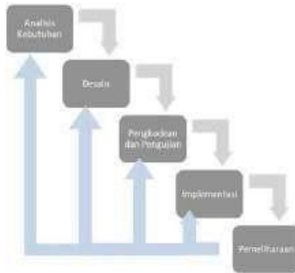
Gambar 1. 1 Model Waterfall
